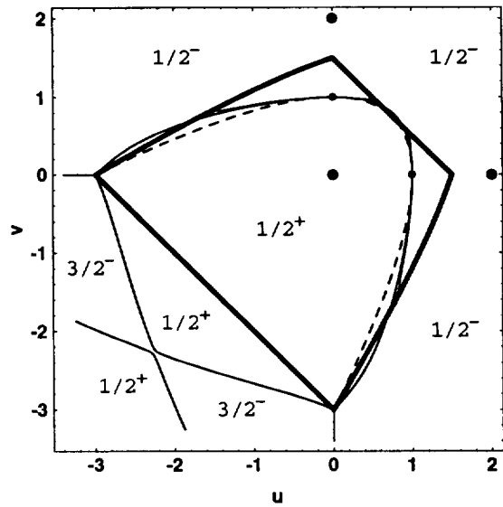
Figure 1. Crossings of the lowest eigenvalues of -D_\mu^2(A) , the Gribov horizon (fat section), \partial\tilde{\Lambda} (dashed curves), \partial\Lambda (thin lines), classical vacua (large dots) and the sphalerons (smaller dots).
