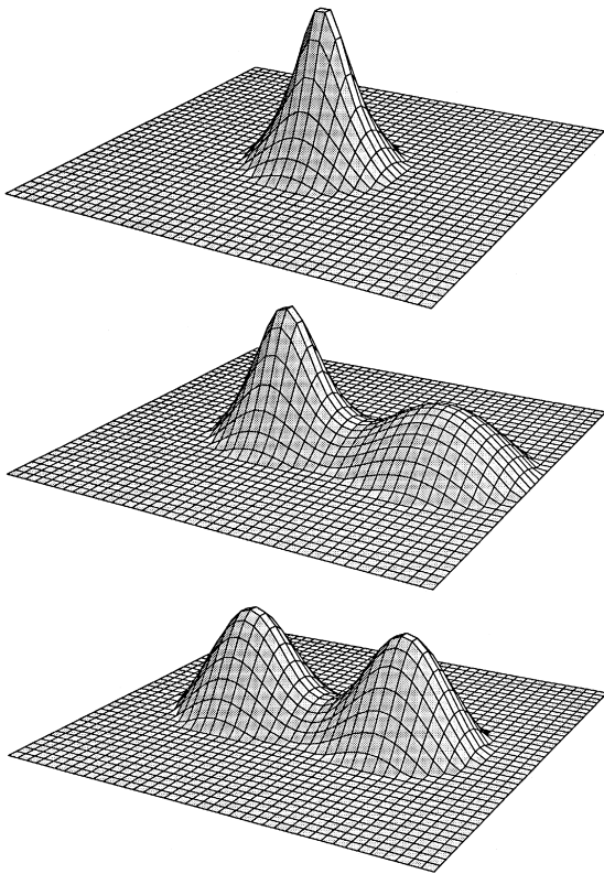
Fig. 1. Profiles for calorons at \omega = 0, 0.125, 0.25 (from top to bottom) with \rho = 1 . The axis connecting the lumps, separated by a distance \pi (for \omega \neq 0 ), corresponds to the direction of \hat{\omega} . The other direction indicates the distance to this axis, making use of the axial symmetry of the solutions. Vertically is plotted the action density, at the time of its maximal value, on equal logarithmic scales for the three profiles. The profiles were cut off at an action density below 1/e . The mass ratio of the two lumps is approximately \omega/\bar{\omega} , i.e. zero (no second lump), a third and one (equal masses), for the respective values of \omega .
